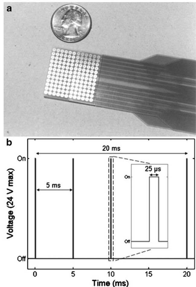
Fig. 2 Tongue stimulation device and CN-NINM waveform. a The 12×12 electrode array, here shown next to a quarter for reference, is placed on the anterior surface of the tongue and is held in place by pressure of the tongue to the roof of the mouth. b CN-NINM stimulation consists of three square-wave pulse bursts with a 200 Hz intraburst and 50 Hz interburst frequency. The stimulation voltage is adjusted at the start of every stimulation session and has a maximum of 24 V
